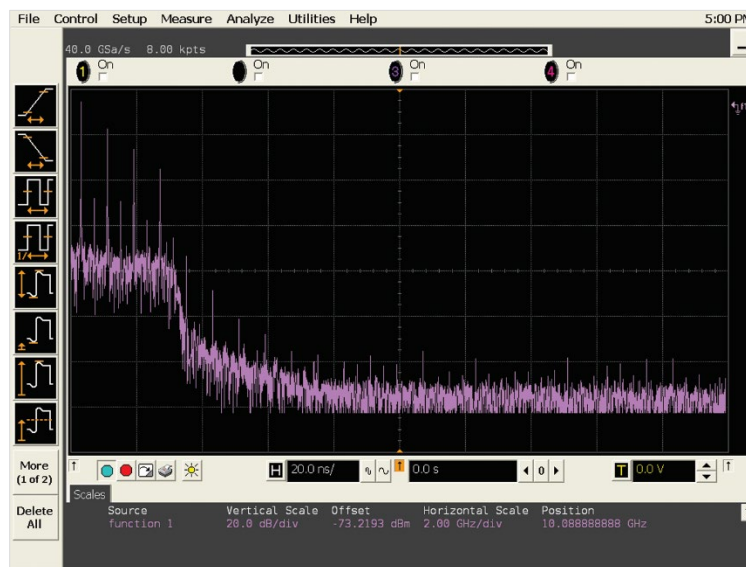
Figure 16a. FFT analysis on a 400-MHz clock using a Keysight Infiniium 3-GHz bandwidth oscilloscope.
