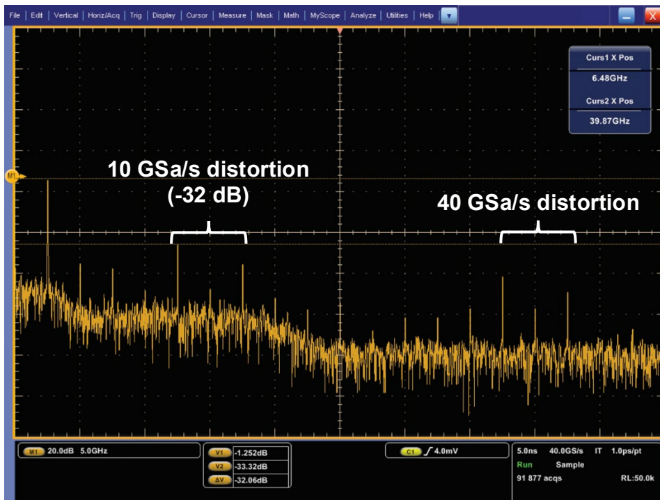
Figure 14b. FFT analysis of 2.5 GHz sine wave captured on another vendor's oscilloscope sampling at 40 GSa/s.
