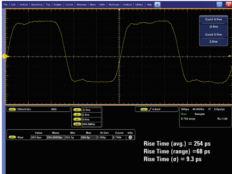
Figure 15b. 400 MHz clock captured on another vendor’s oscilloscope 2.5 GHz oscilloscope sampling at 40 GSa/s.
