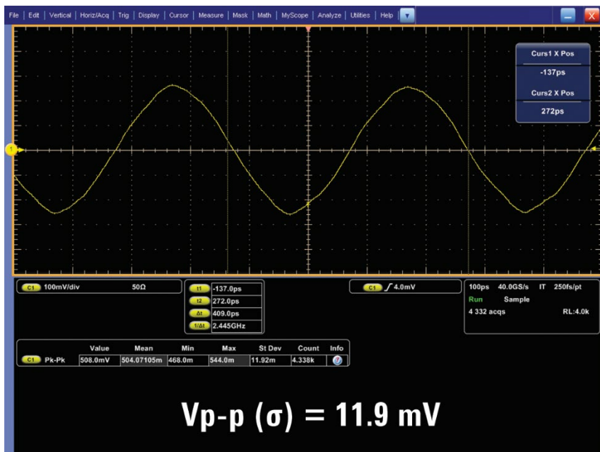
Figure 13b. 2.5 GHz sine wave captured on another vendor's oscilloscope 2.5 GHz bandwidth oscilloscope sampling at 40 GSa/s (interleaved).
