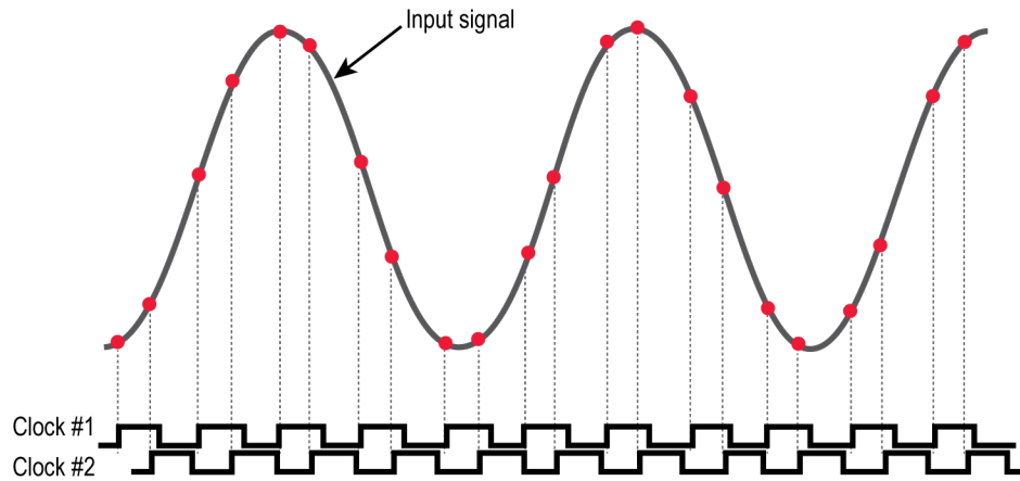
Figure 9. Timing diagram showing non-evenly spaced samples.
