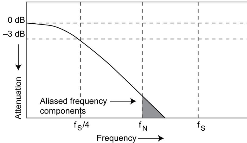
Figure 5. Limiting oscilloscope bandwidth ( f_{BW} ) to 1/4 the sample rate ( f_s/4 ) reduces frequency components above the Nyquist frequency ( f_N ).
