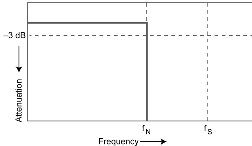
Figure 2. Theoretical brick-wall frequency response.
