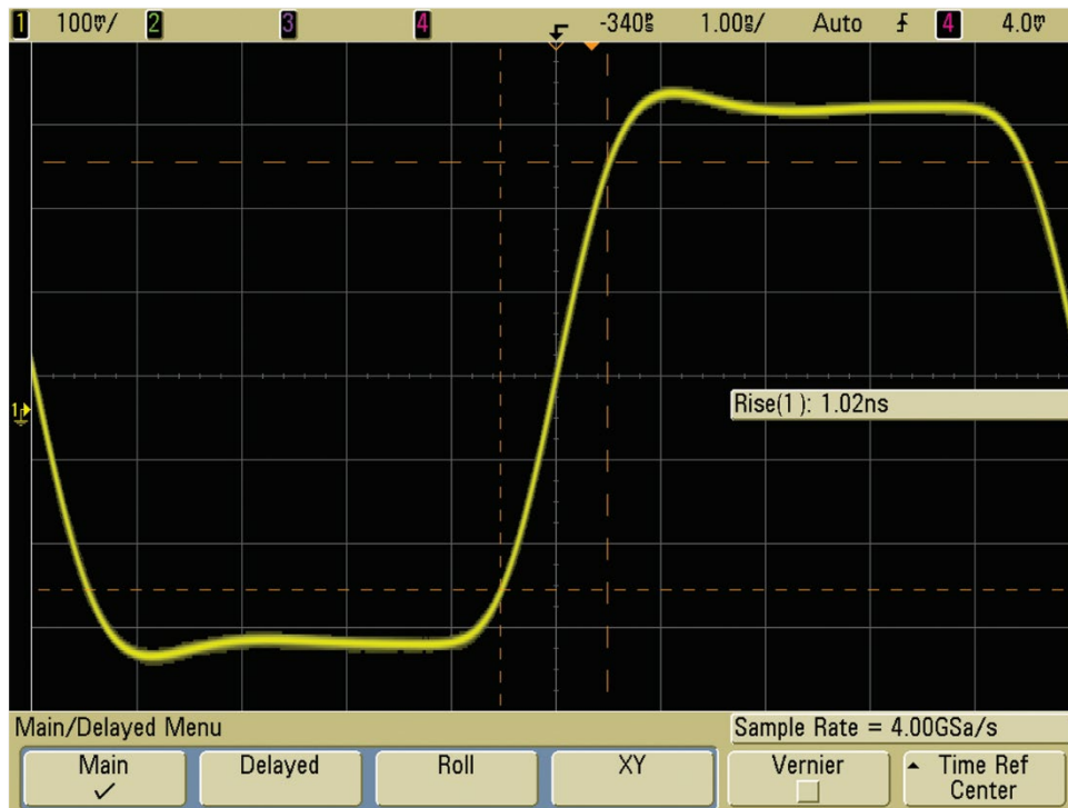
Figure 7. Keysight 500-MHz bandwidth scope sampling at 4 GSa/s produces minimal.
