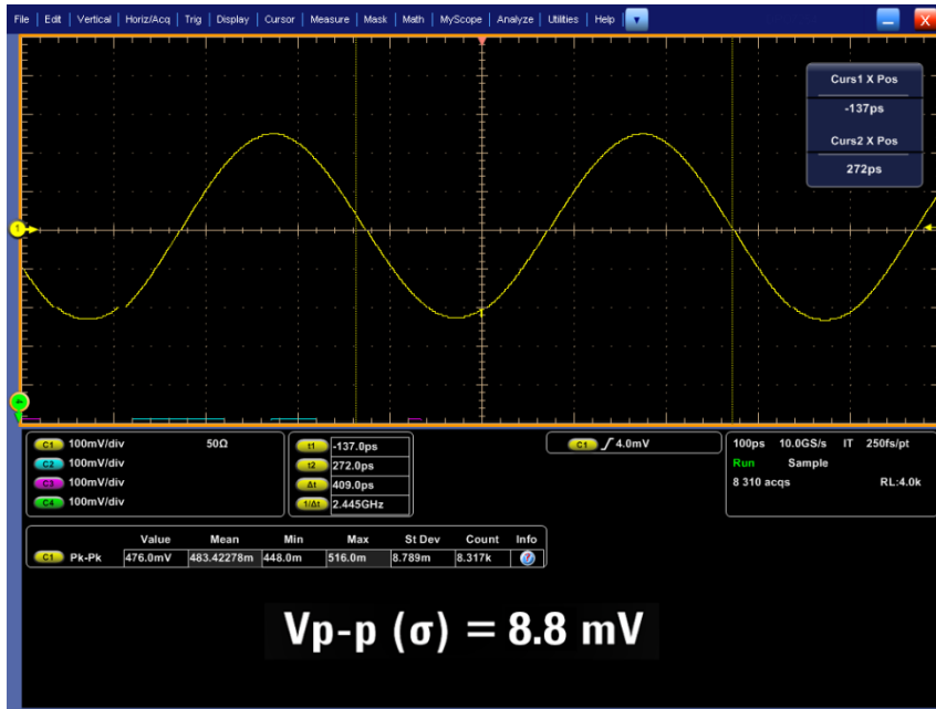
Figure 13a. 2.5 GHz sine wave captured on another vendor's oscilloscope 2.5 GHz bandwidth oscilloscope sampling at 10 GSa/s (non-interleaved).
