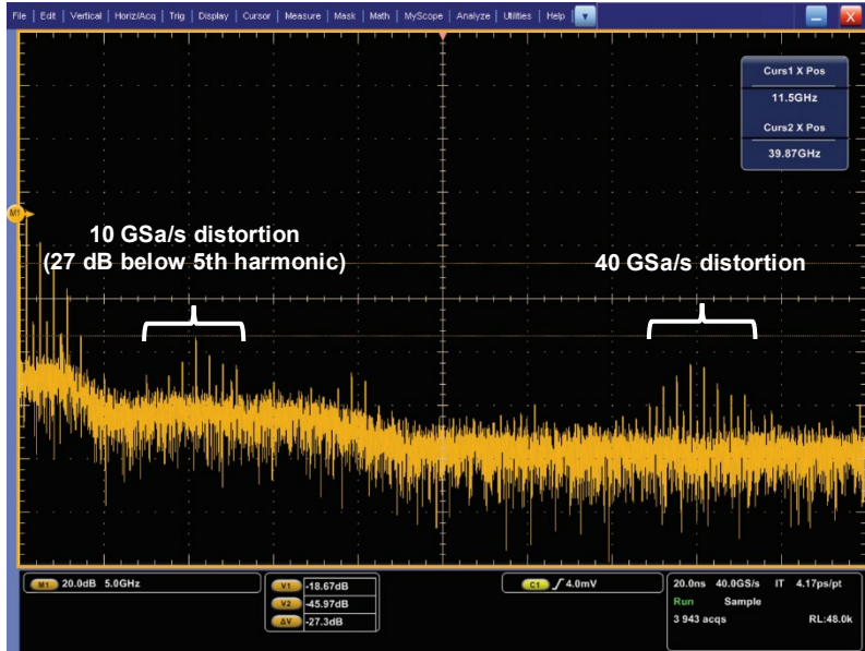
Figure 16b. FFT analysis on a 400-MHz clock using another vendor's oscilloscope 2.5 GHz bandwidth oscilloscope.
