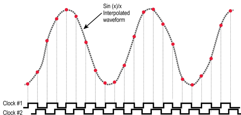
Figure 10. Timing diagram showing distorted reconstruction of waveform using a \text{Sin}(x)/x filter due to poor phase-delayed clocking.
