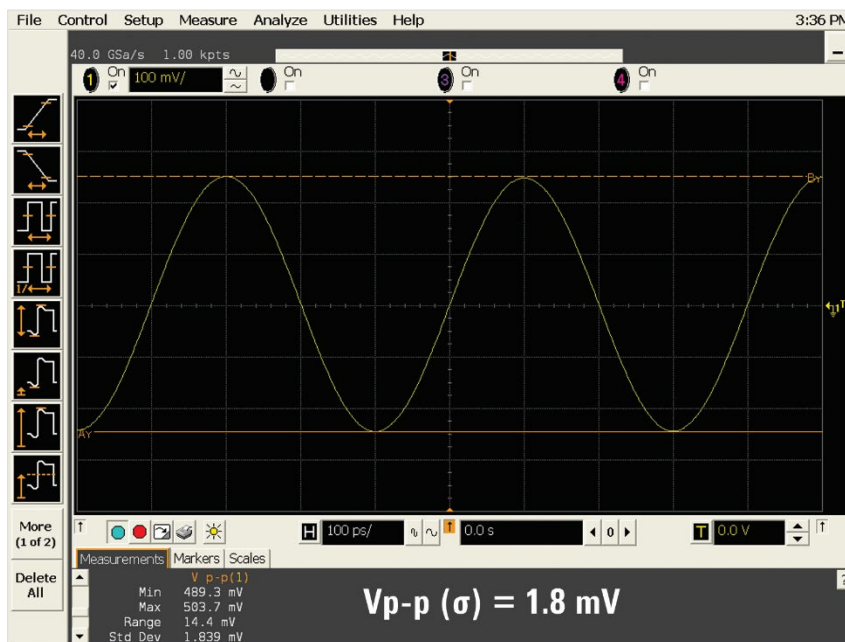
Figure 12b. 2.5 GHz sine wave captured on the Keysight Infiniium oscilloscope sampling at 40 GSa/s (interleaved).
