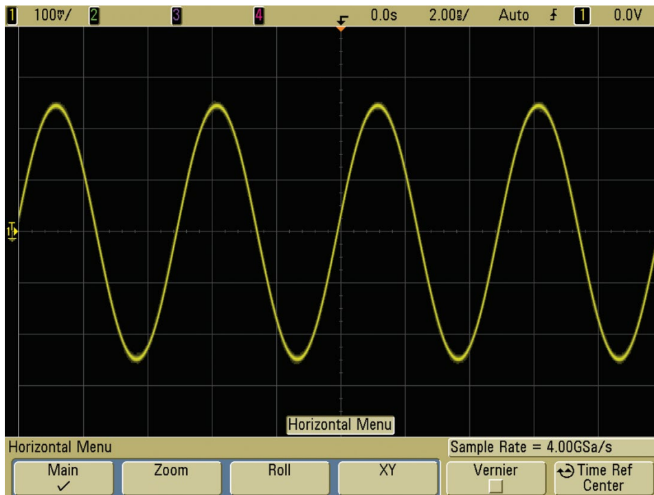
Figure 11a. 200 MHz sine wave captured on a Keysight 1 GHz bandwidth oscilloscope sampling at 4 GSa/s.
