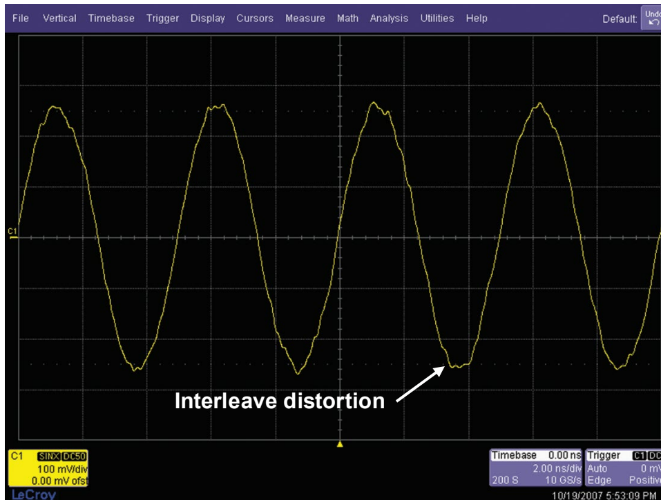
Figure 11b. 200 MHz sine wave captured on another vendor's oscilloscope 1 GHz bandwidth oscilloscope sampling at 10 GSa/s.
