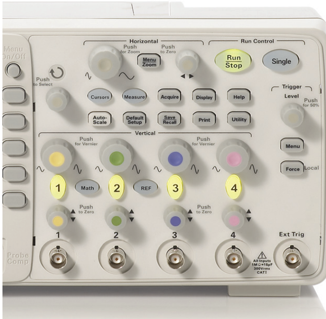
Figure 33. Oscilloscope front panels should include knobs for all key setup variables
