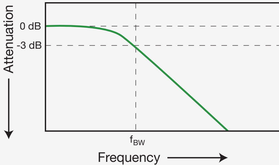
Figure 1. Oscilloscopes exhibit a low-pass frequency response that rolls off higher frequencies
